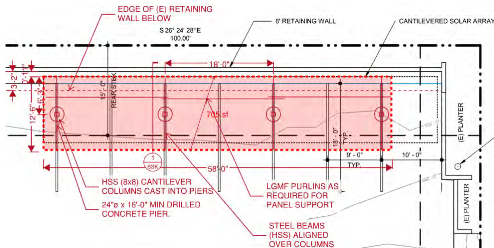
Figure 1 - Conceptual PV Canopy Plan
